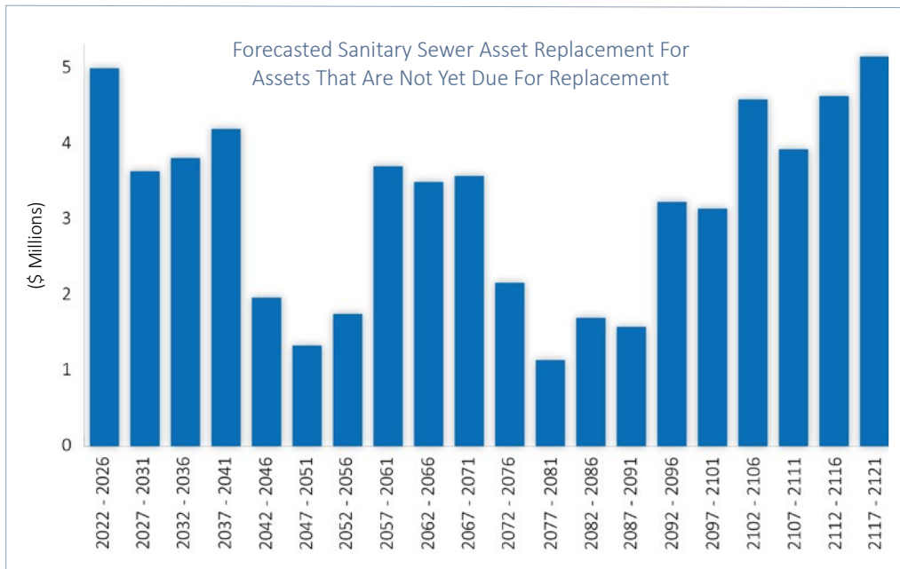
Figure 28: Sanitary Sewer Replacement by Year Range
